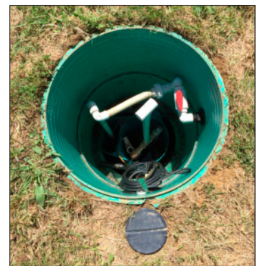
The Orenco high-head effluent pump housed in the pump vault has a life expectancy of over twenty years.
